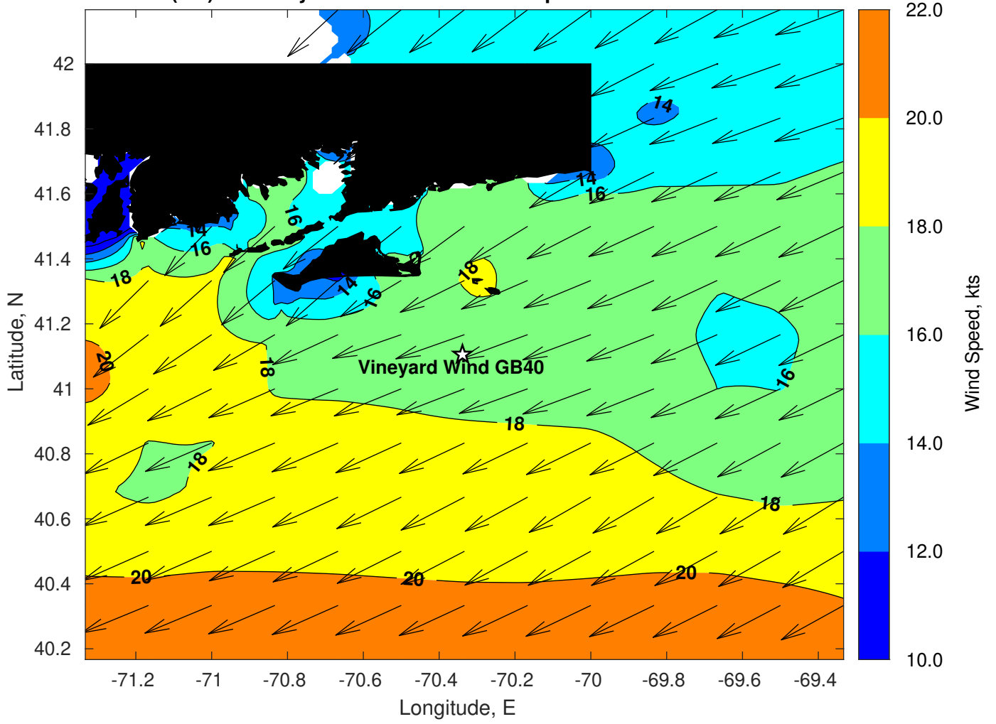
Winds (kts) for Vineyard Wind GB40 at 07-Sep-2022 12:00:00
