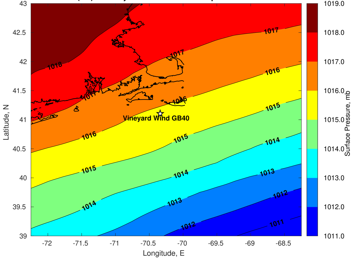
Surface Pressure (mb) for Vineyard Wind GB40 at 09-Sep-2022 12:00:00
