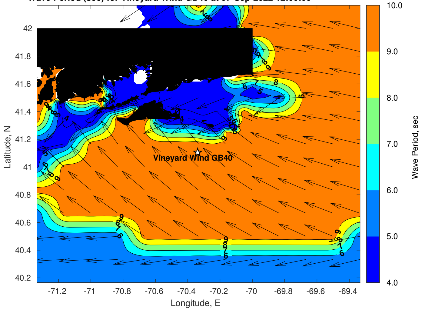
Wave Period (sec) for Vineyard Wind GB40 at 07-Sep-2022 12:00:00
