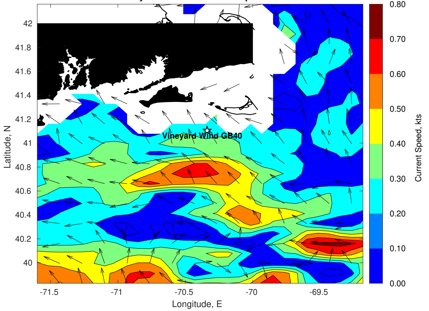
Surface Currents for Vineyard Wind GB40 at 07-Sep-2022 00:00:00
