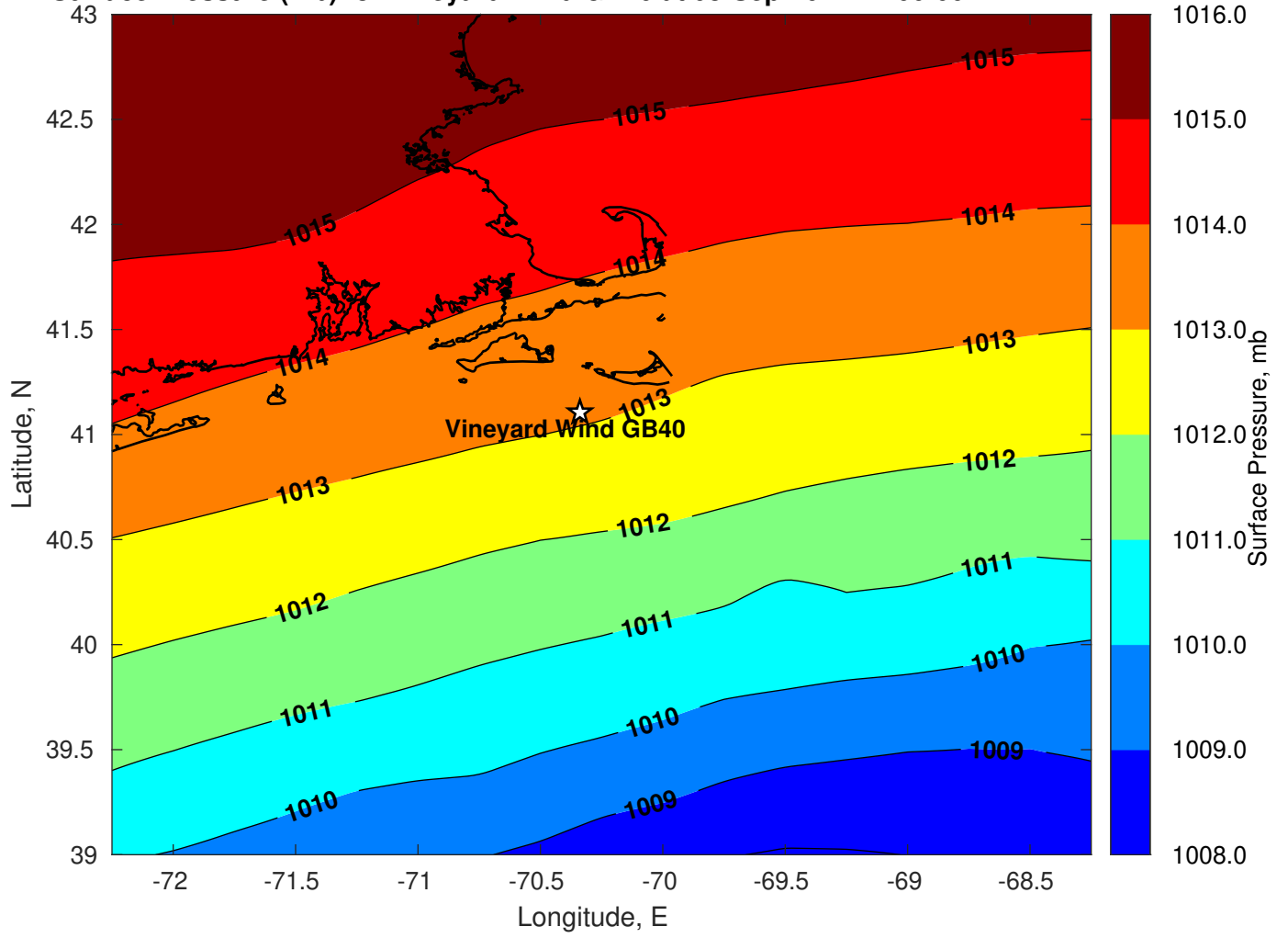
Surface Pressure (mb) for Vineyard Wind GB40 at 08-Sep-2022 12:00:00
