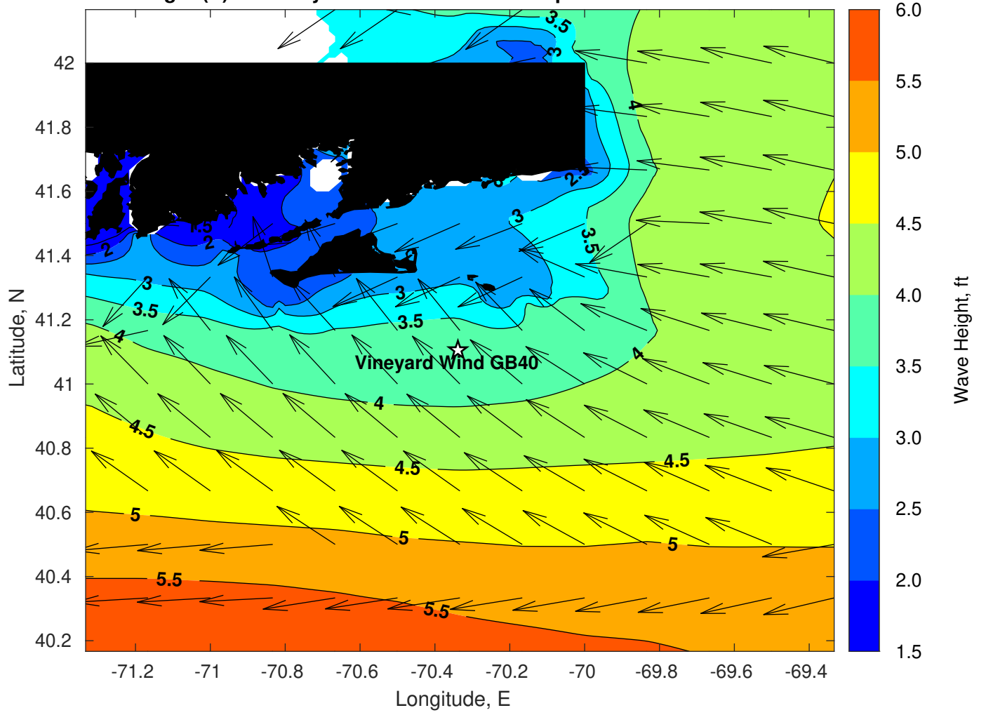
Wave Height (ft) for Vineyard Wind GB40 at 07-Sep-2022 12:00:00
