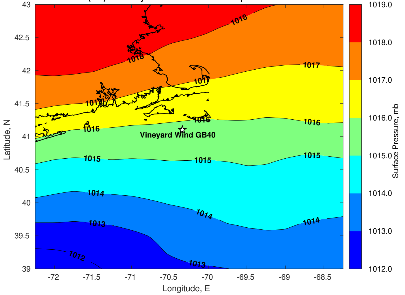
Surface Pressure (mb) for Vineyard Wind GB40 at 07-Sep-2022 12:00:00
